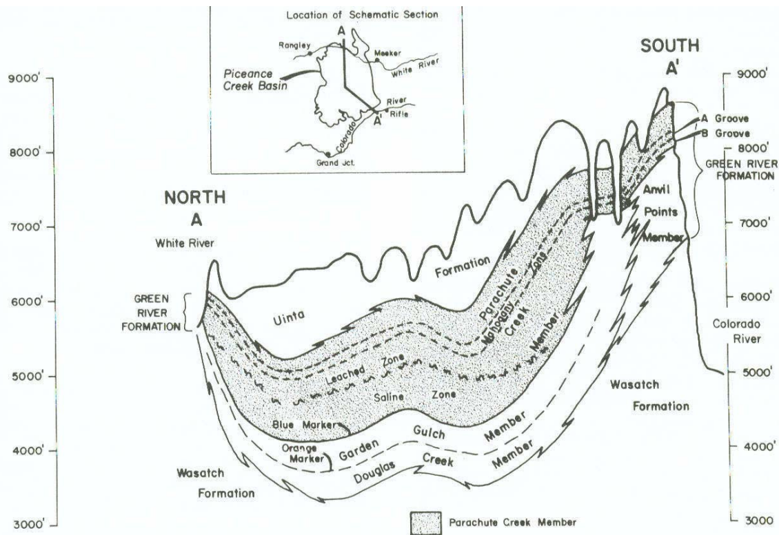
Figure 2 Oil shale members of the Green River Formation Synthetic Fuels Data Handbook , Cameron Engineers, Inc., 1978, p.7
